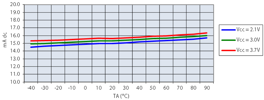
Current consumption in RX vs. temperature
